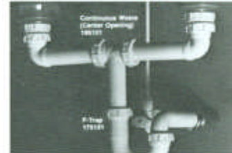
Center Outlet Waste w/Wall Mount Trap
