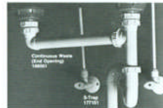
End Outlet Waste w/Floor Mount Trap
