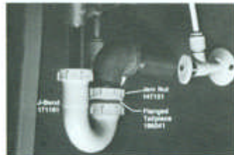
Wall Mount Trap for Cast Elbow
