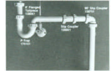
Single Sink or Vanity
