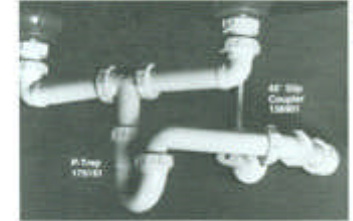
Double Sink or Vanity
