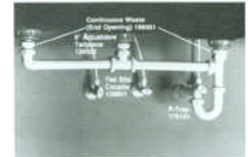
Multiple Sink or Vanity
