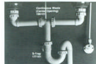
Center Outlet Waste w/Floor Mount Trap
