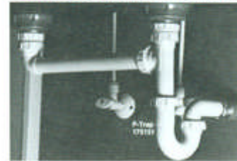
End Outlet Waste w/Wall Mount Trap
