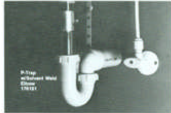
Wall Mount Trap (solvent weld type)
